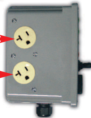
Side View Showing Receptacles
