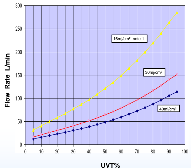
UVD1200 Performance Curves note 2
